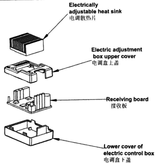
3301 Receiving board group 接收板组
