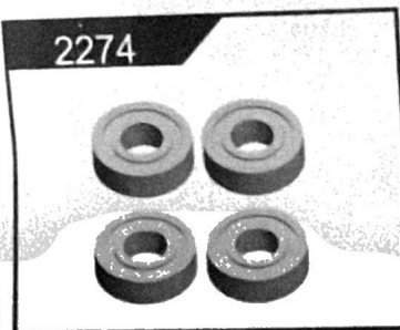
6.35*9.525*3.175 bearing 6.35*9.525*3.175轴承组
