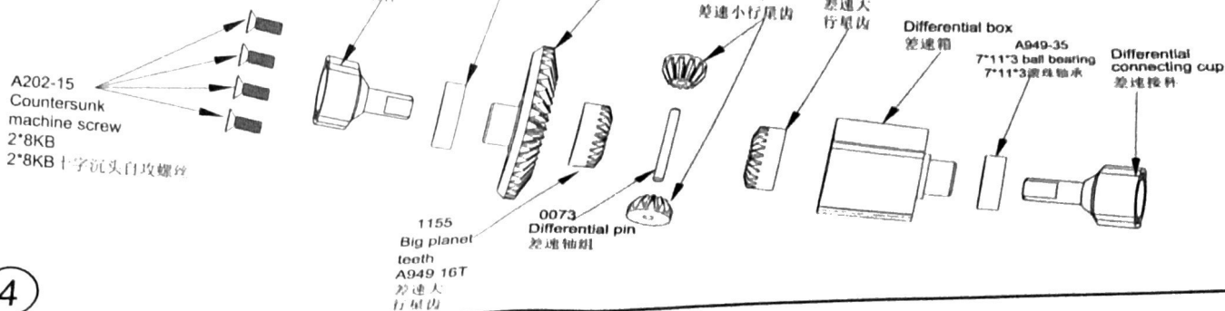
2990 Differential components 差速器组件
