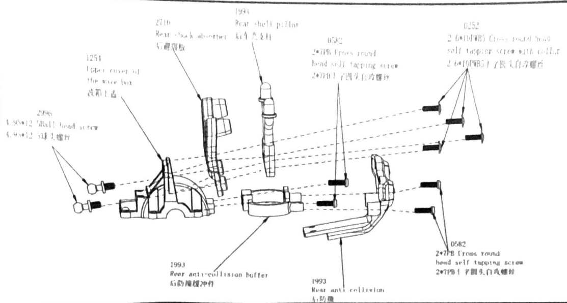
Rear wave box upper cover group 后波箱上盖组
